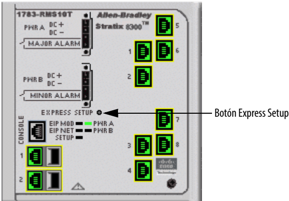
Switch Stratix 8000/8300
