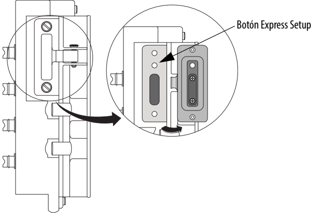
Switch Stratix 8000/8300
