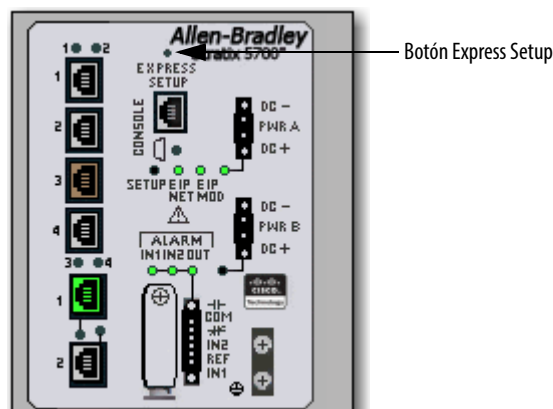
Switch Stratix 5700
